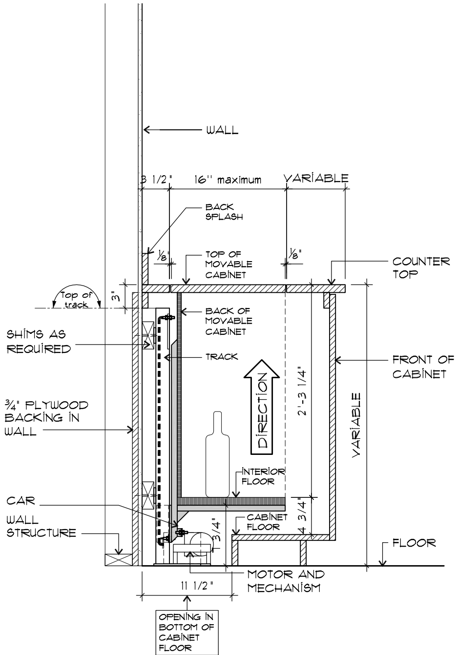
SIDE ELEVATION BOTTOM POSITION
