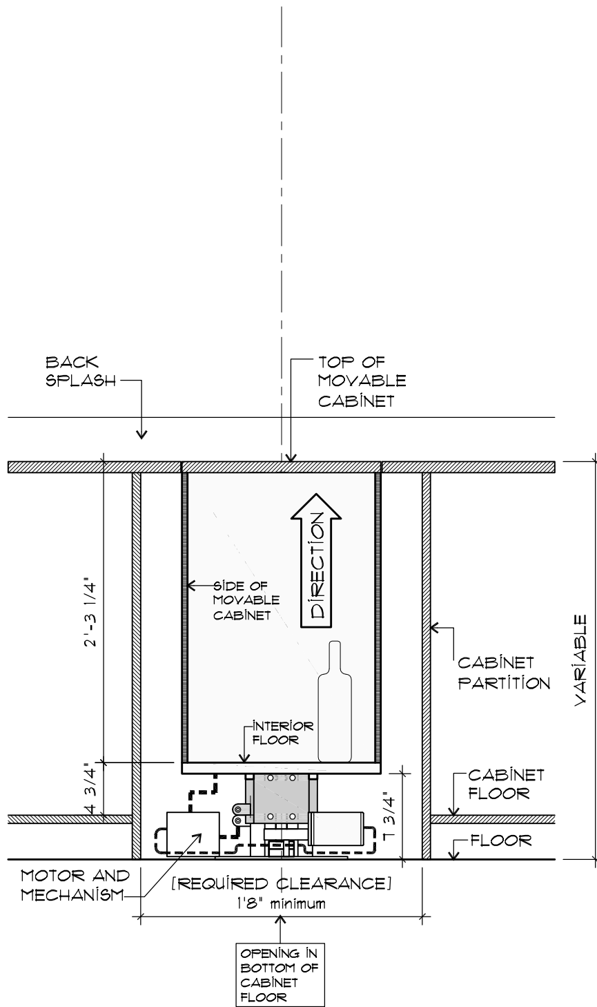
FRONT ELEVATION BOTTOM POSITION
