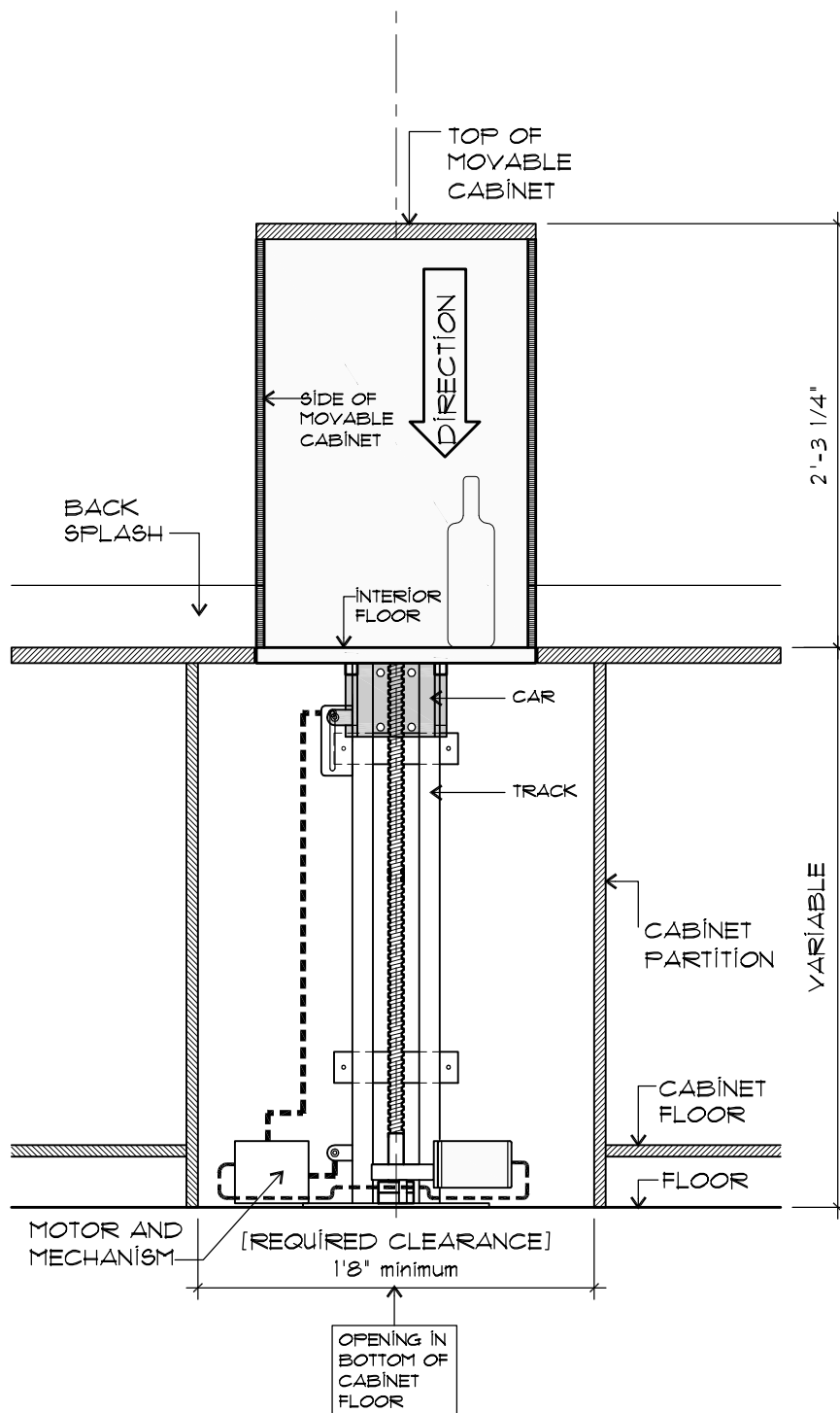
FRONT ELEVATION TOP POSITION
