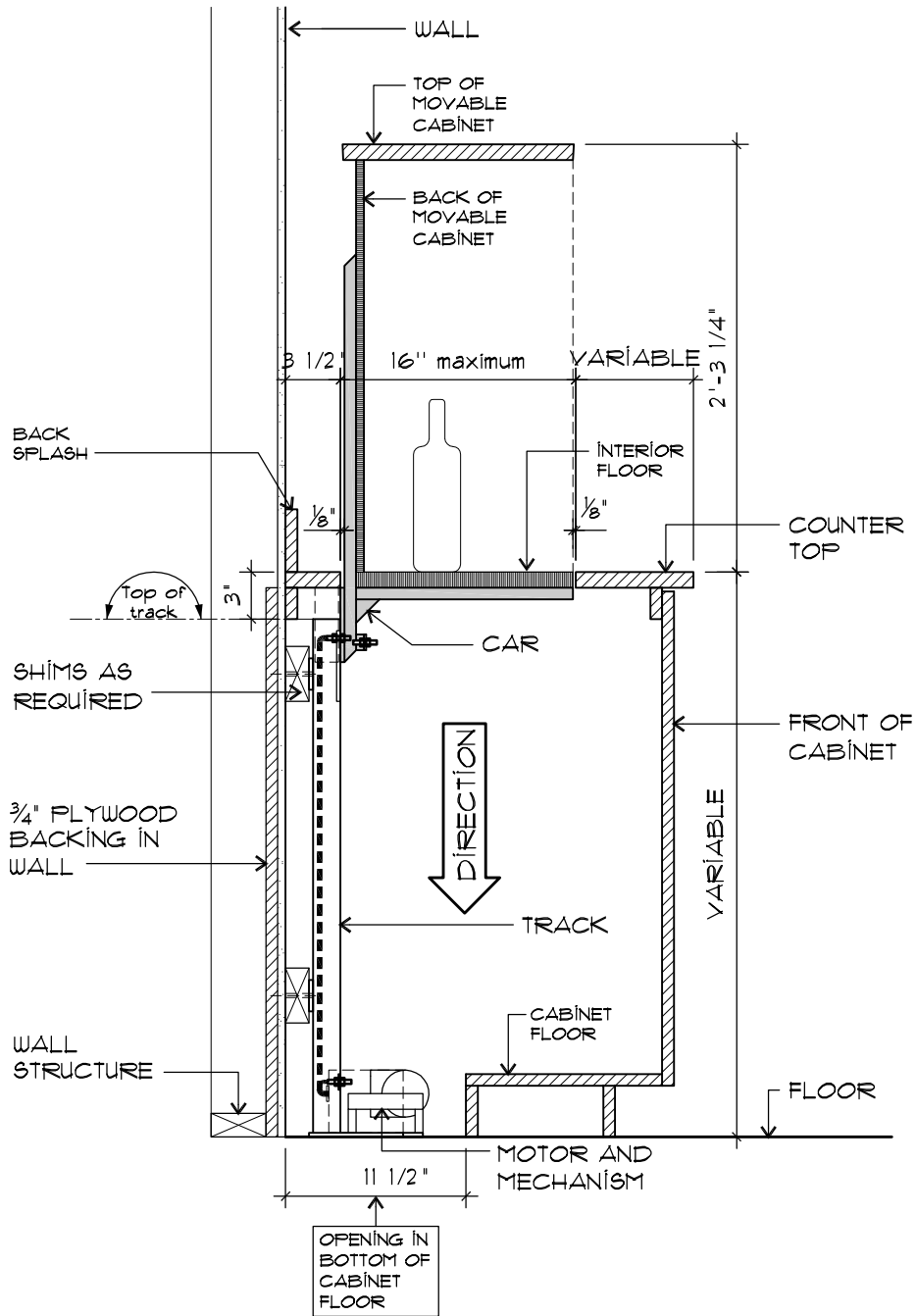
SIDE ELEVATION TOP POSITION
